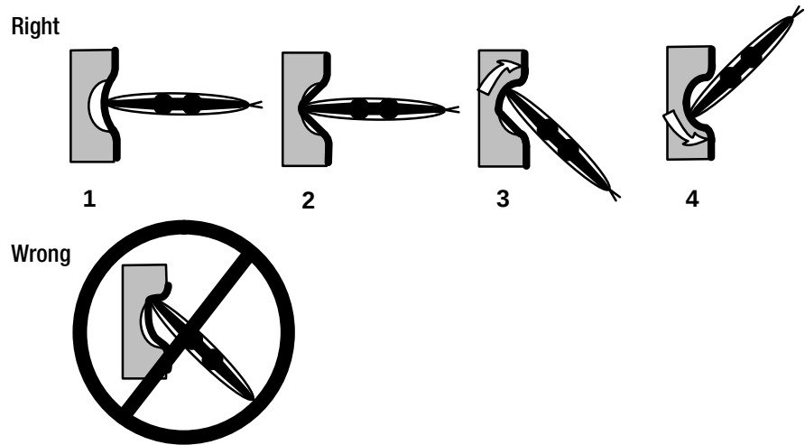
FIGURE 1 Technique For Stretching Heated Film into Channels
