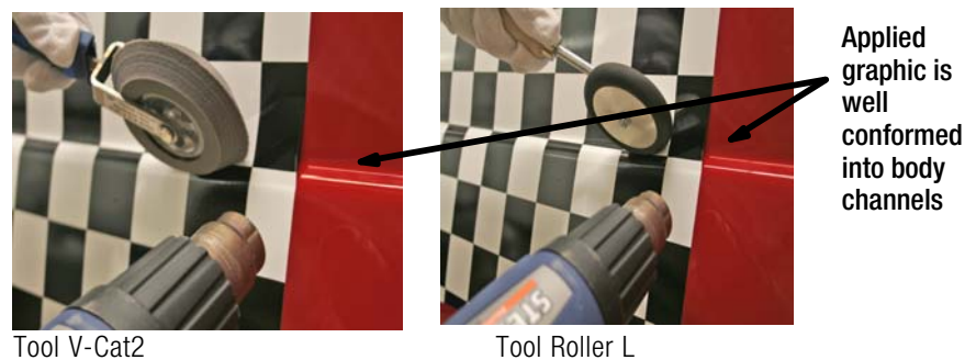
FIGURE 2 Technique For Stretching Heated Film into Channels
